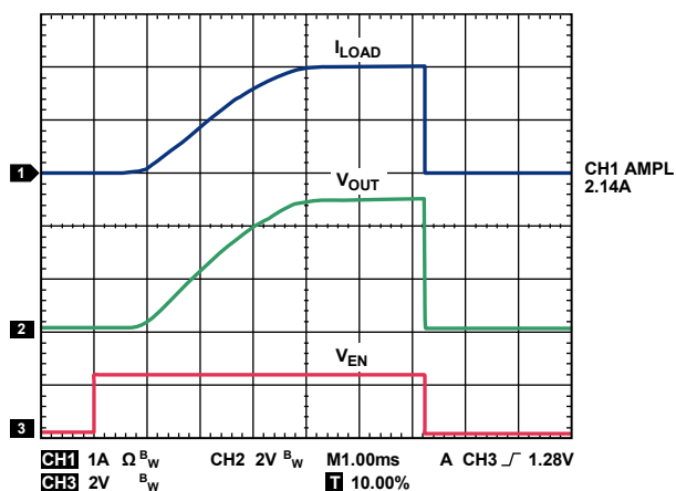
Figure 21. Typical Turn-On Time and Inrush Current, V_{IN} = 5.5\text{ V} , 2 A Load
