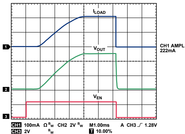
Figure 20. Typical Turn-On Time and Inrush Current, V_{IN} = 5.5\text{ V} , 200 mA Load
