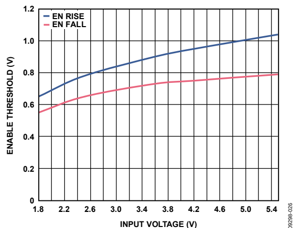
Figure 28. Typical EN Threshold vs. Input Voltage ( V_{\text{IN}} )
