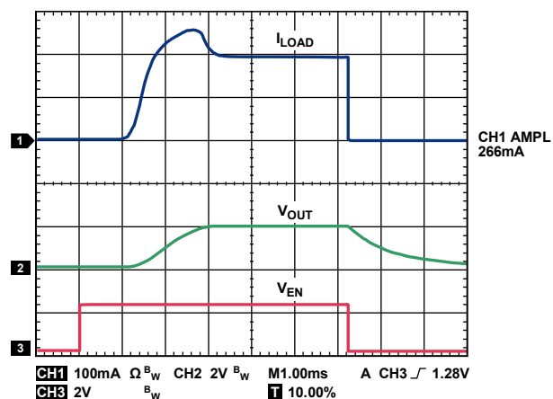
Figure 18. Typical Turn-On Time and Inrush Current, V_{IN} = 1.9\text{ V} , 200 mA Load, C_{OUT} = 100\text{ }\mu\text{F}
