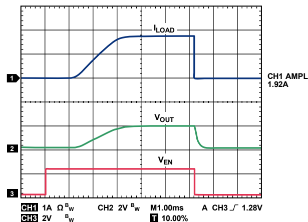
Figure 19. Typical Turn-On Time and Inrush Current, V_{IN} = 1.9\text{ V} , 2 A Load, C_{OUT} = 100\text{ }\mu\text{F}
