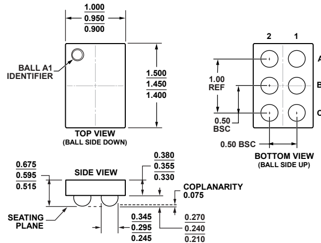
Figure 34. 6-Ball Wafer Level Chip Scale Package [WLCSP] (CB-6-2)
