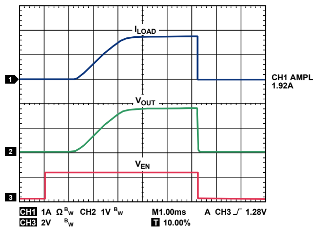
Figure 17. Typical Turn-On Time and Inrush Current, V_{IN} = 1.9\text{ V} , 2 A Load
