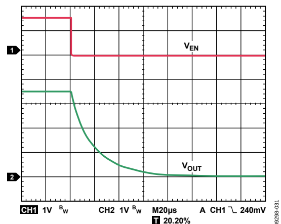
Figure 33. Typical Turn-Off Time
