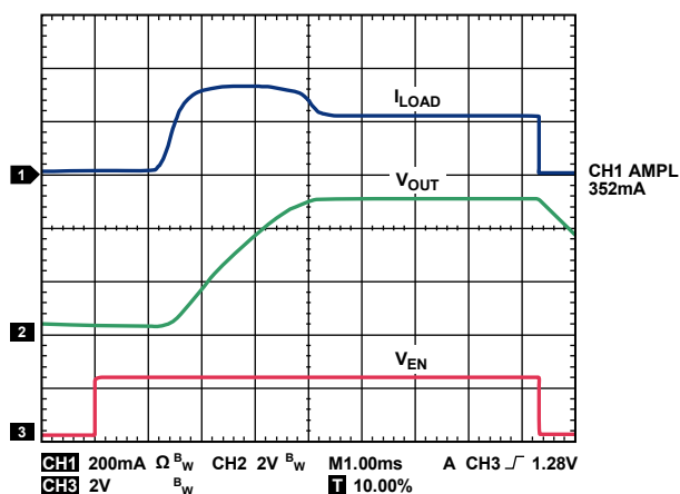
Figure 22. Typical Turn-On Time and Inrush Current, V_{IN} = 5.5\text{ V} , 200 mA Load, C_{OUT} = 100\text{ }\mu\text{F}
