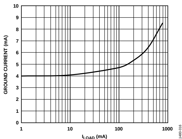
Figure 16. Ground Current vs. Load Current ( I_{LOAD} ), ADM7151-04, V_{OUT} = 5\text{ V}
