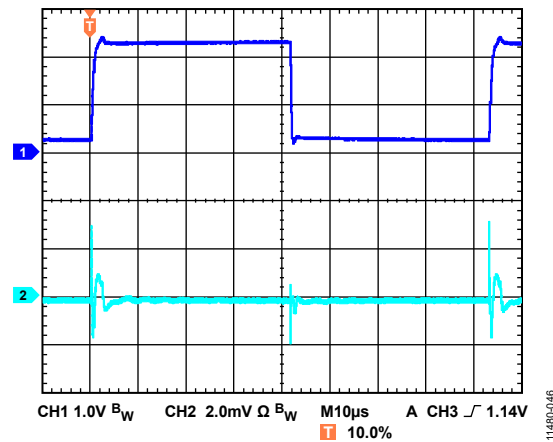
Figure 46. Line Transient Response, 2\text{ V} Input Step, I_{LOAD} = 800\text{ mA} , V_{OUT} = 5\text{ V} , V_{IN} = 6.2\text{ V} , CH1 = V_{IN} , CH2 = V_{OUT}
