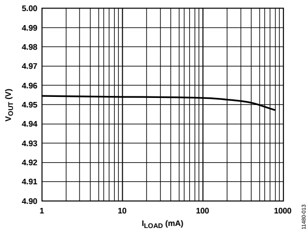
Figure 13. Output Voltage ( V_{OUT} ) vs. Load Current ( I_{LOAD} ), ADM7151-04, V_{OUT} = 5\text{ V}
