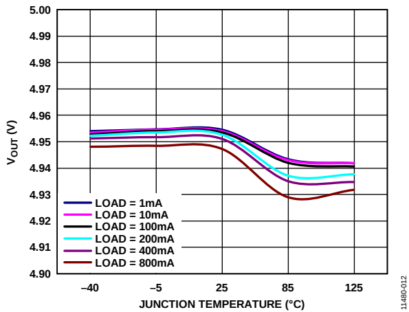
Figure 12. Output Voltage ( V_{OUT} ) vs. Junction Temperature ( T_J ), ADM7151-04, V_{OUT} = 5\text{ V}
