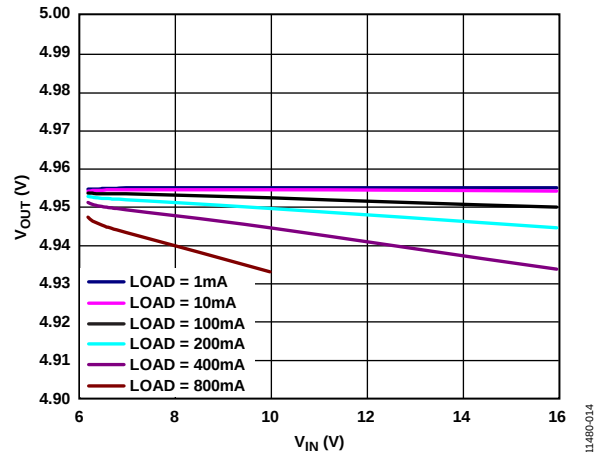
Figure 14. Output Voltage ( V_{OUT} ) vs. Input Voltage ( V_{IN} ), ADM7151-04, V_{OUT} = 5\text{ V}
