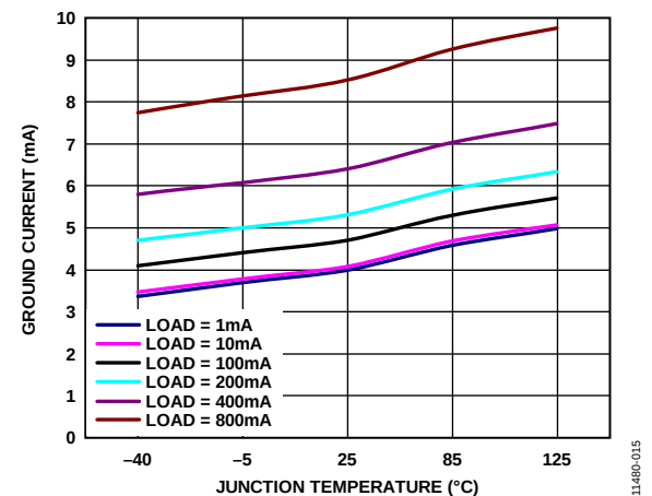
Figure 15. Ground Current vs. Junction Temperature ( T_J ), ADM7151-04, V_{OUT} = 5\text{ V}
