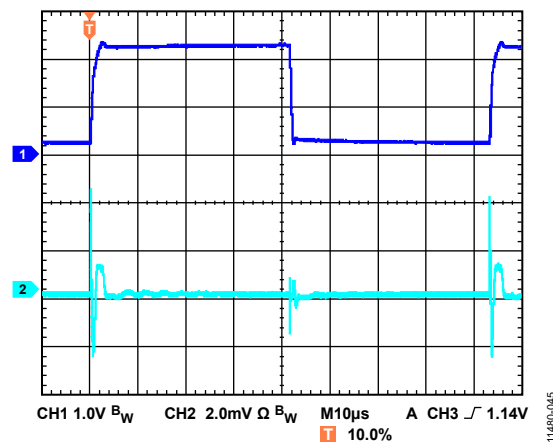
Figure 45. Line Transient Response, 2\text{ V} Input Step, I_{LOAD} = 800\text{ mA} , V_{OUT} = 3.3\text{ V} , V_{IN} = 4.5\text{ V} , CH1 = V_{IN} , CH2 = V_{OUT}
