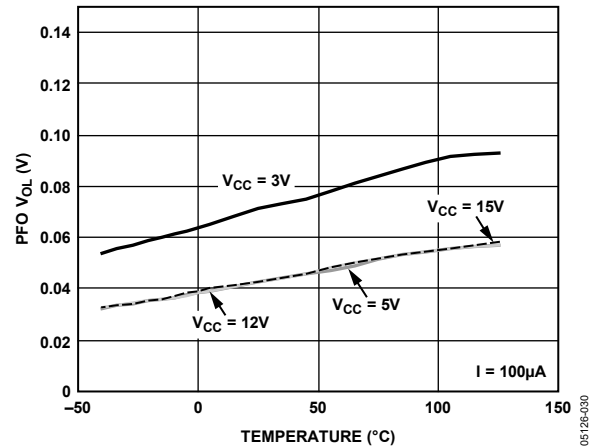
Figure 36. PFO Output Low Voltage vs. Temperature, I = 100\mu\text{A}
