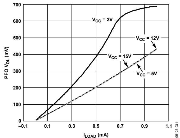
Figure 37. PFO Output Low Voltage vs. Load Current
