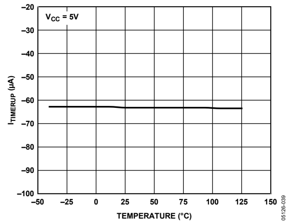
Figure 15. I_{TIMERUP} (During Cct Breaker Delay) vs. Temperature
