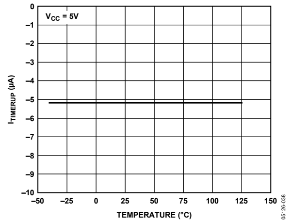
Figure 13. I_{TIMERUP} (In Initial Cycle) vs. Temperature
