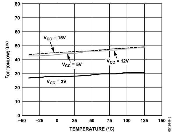
Figure 25. t_{\text{OFF(ONLOW)}} vs. Temperature
