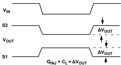
Figure 21. Charge Injection
