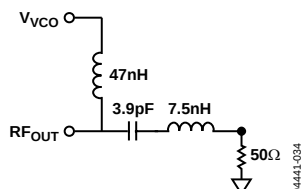
Figure 30. Optimum ADF4360-7 Output Stage
