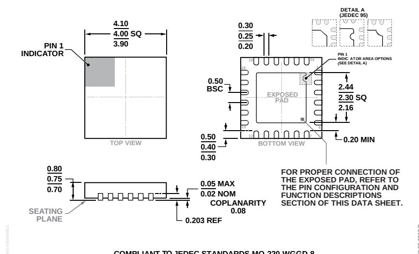
Figure 32. 24-Lead Lead Frame Chip Scale Package [LFCSP] 4 mm × 4 mm and 0.75 mm Package Height (CP-24-14) Dimensions shown in millimeters
