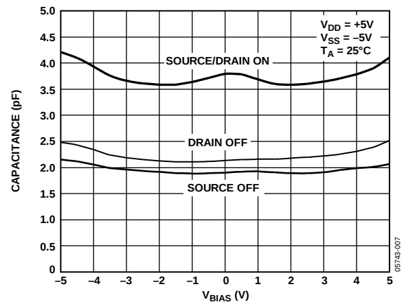
Figure 23. Capacitance vs. Source Voltage for Dual Supply
