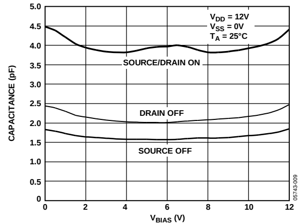
Figure 22. Capacitance vs. Source Voltage for Single Supply
