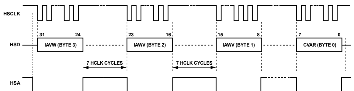
Figure 94. HSDC Communication for HSIZE = 1, HGAP = 1, HXFER[1:0] = 00, and HSAPO[0] = 0
