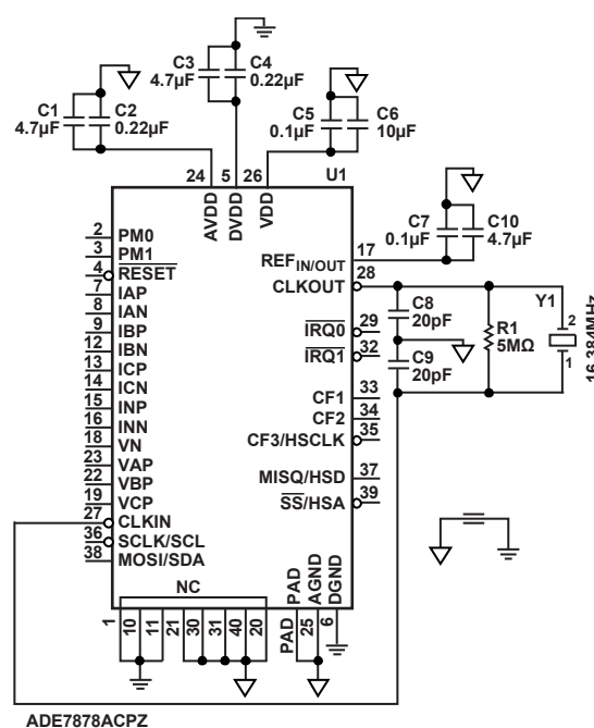
Figure 95. ADE7878 Crystal and Capacitors Connections
