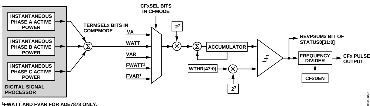
Figure 75. Energy-to-Frequency Conversion
