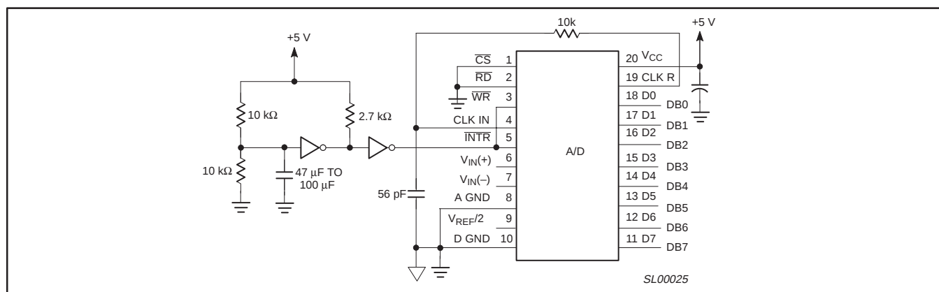
Figure 10. Connection for Continuous Conversion
