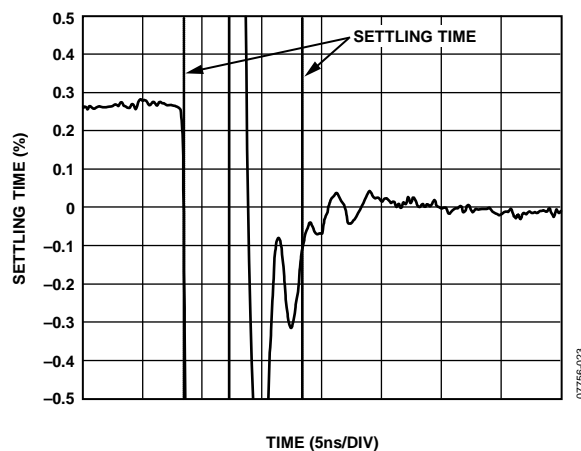
Figure 24. 0.1% Short-Term Settling Time
