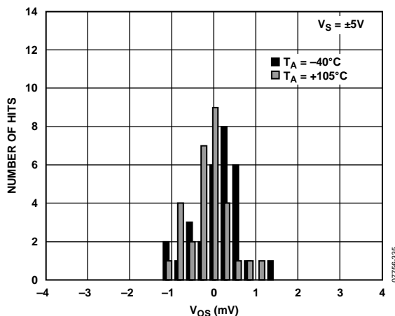
Figure 33. Input Offset Voltage Histogram over Temperature ( V_S = \pm 5\text{ V} , LFCSP Only)
