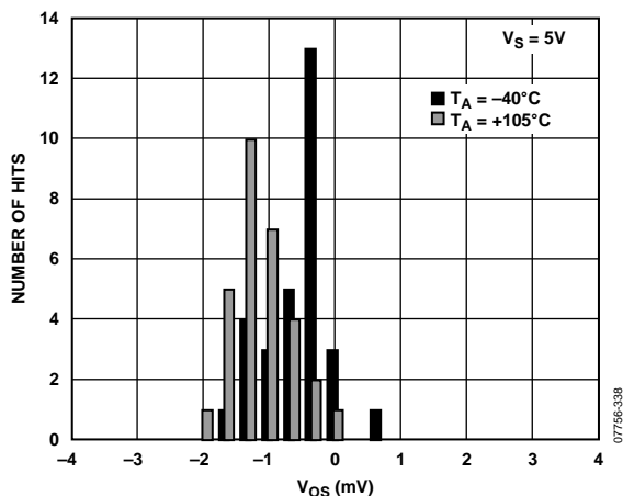
Figure 36. Input Offset Voltage Histogram over Temperature ( V_S = 5\text{ V} , LFCSP Only)
