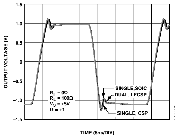
Figure 23. Large Signal Transient Response vs. Package
