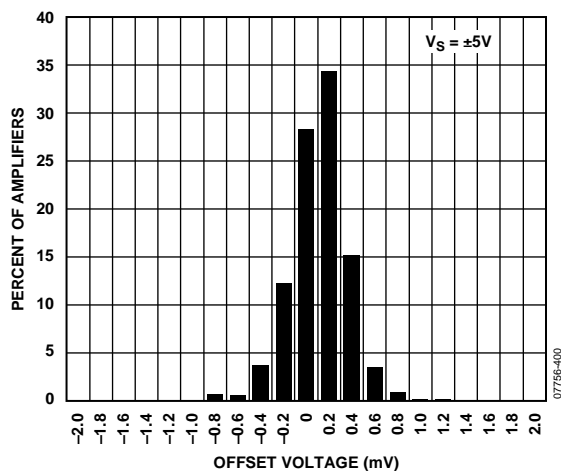
Figure 32. Input Offset Voltage Histogram ( V_S = \pm 5\text{ V} , LFCSP Only)
