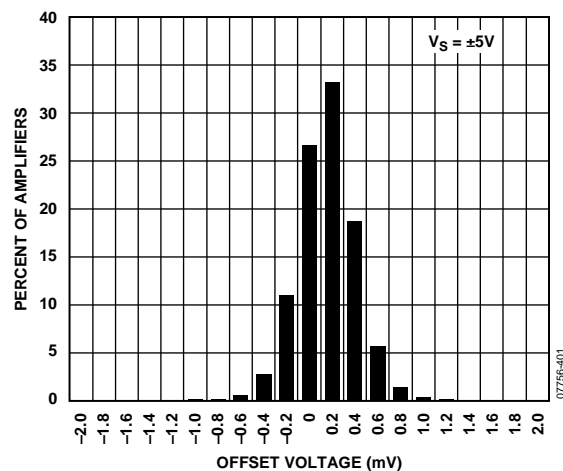
Figure 35. Input Offset Voltage Histogram ( V_S = \pm 5\text{ V} , SOIC Only)
