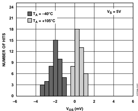
Figure 37. Input Offset Voltage Histogram over Temperature ( V_S = 5\text{ V} , SOIC Only)
