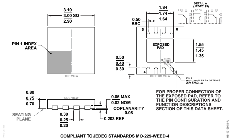
Figure 71. 8-Lead Lead Frame Chip Scale Package [LFCSP] 3 mm × 3 mm Body and 0.75 mm Package Height (CP-8-13)
