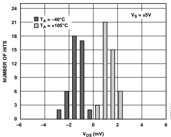
Figure 34. Input Offset Voltage Histogram over Temperature ( V_S = \pm 5\text{ V} , SOIC Only)
