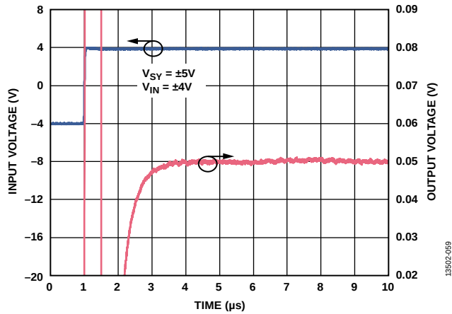
Figure 63. Positive Settling Time, A_V = -10 , V_{SY} = \pm 5\text{ V}
