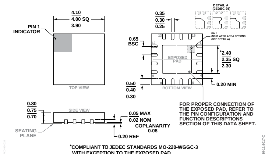
Figure 108. 16-Lead Lead Frame Chip Scale Package [LFCSP] 4 mm × 4 mm Body and 0.75 mm Package Height (CP-16-20)
