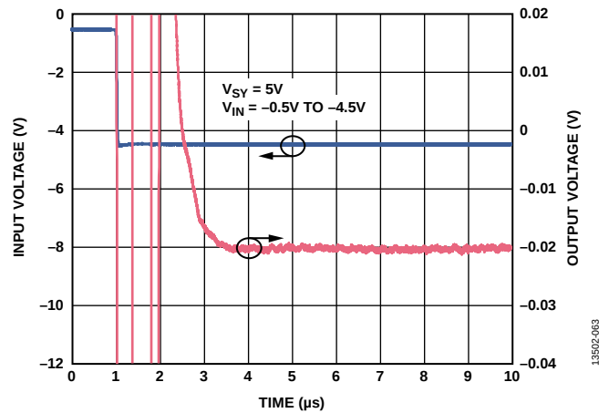
Figure 67. Negative Settling Time, A_V = -10 , V_{SY} = 5\text{ V}
