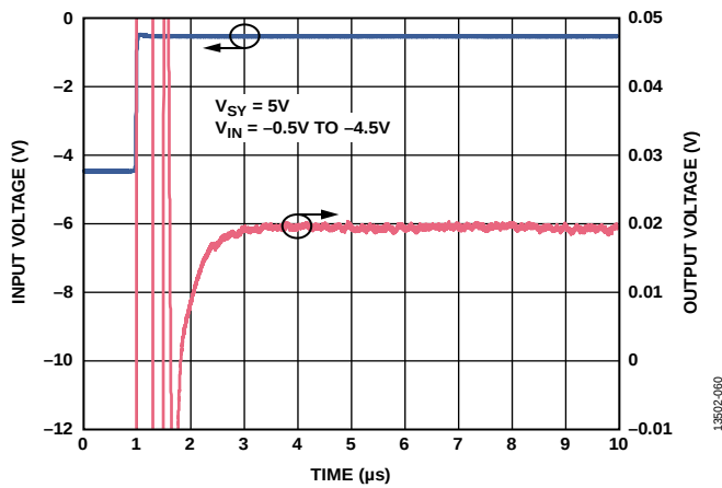
Figure 64. Positive Settling Time, A_V = -10 , V_{SY} = 5\text{ V}
