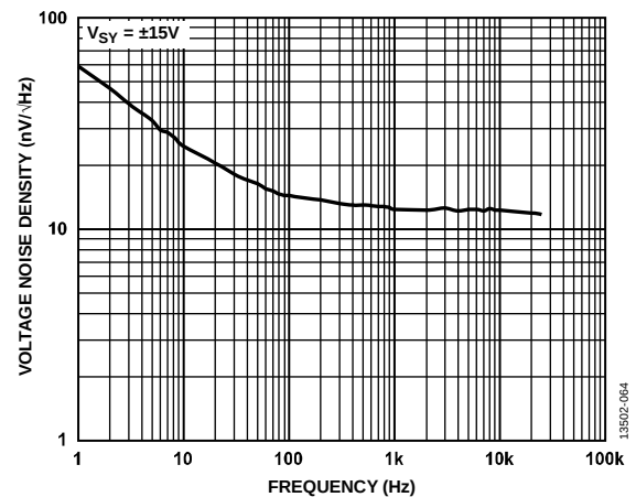
Figure 68. Voltage Noise Density, V_{SY} = \pm 15\text{ V}
