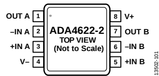
Figure 4. 8-Lead MSOP Pin Configuration, ADA4622-2
