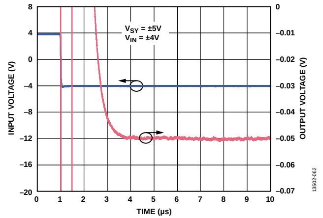
Figure 66. Negative Settling Time, A_V = -10 , V_{SY} = \pm 5\text{ V}
