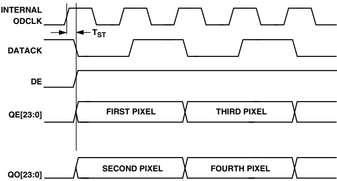
Figure 35. 2 Pixels per Clock (DATAACK Inverted)
