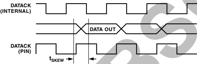
Figure 31. DVI Output Timing
