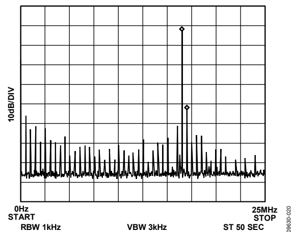
Figure 20. f_{CLK} = 50 MHz, f_{OUT} = 16.5 MHz. Frequency Word = 547AE148
