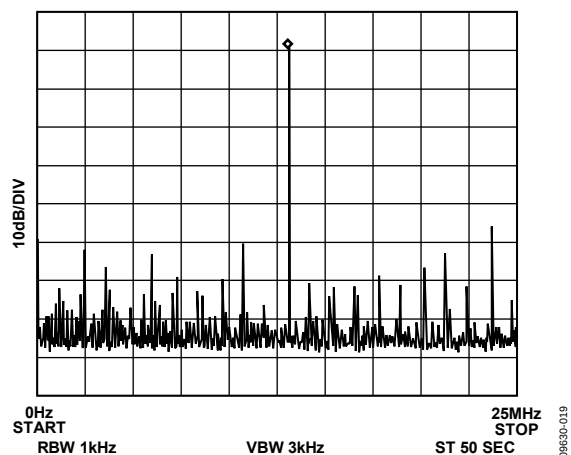
Figure 19. f_{CLK} = 50 MHz, f_{OUT} = 13.1 MHz. Frequency Word = 43126E98
