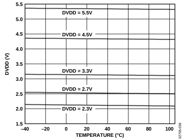
Figure 17. SIGN BIT OUT High Level, I_{SINK} = 1 \text{ mA}
