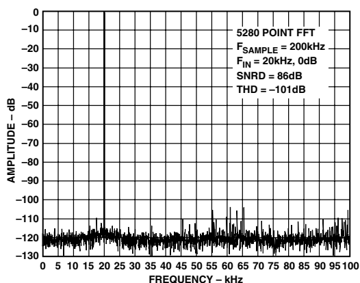
Figure 17. FFT Plot
