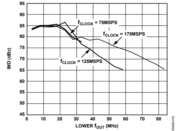
Figure 17. Dual-Tone IMD vs. Lower f_{OUT} and f_{CLOCK} @ 0 dBFS
