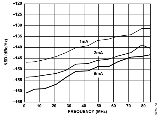
Figure 16. NSD vs. f_{OUT} and I_{OUTES} @ 175 MSPS
