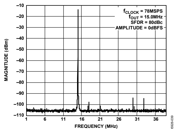
Figure 24. Single-Tone SFDR
