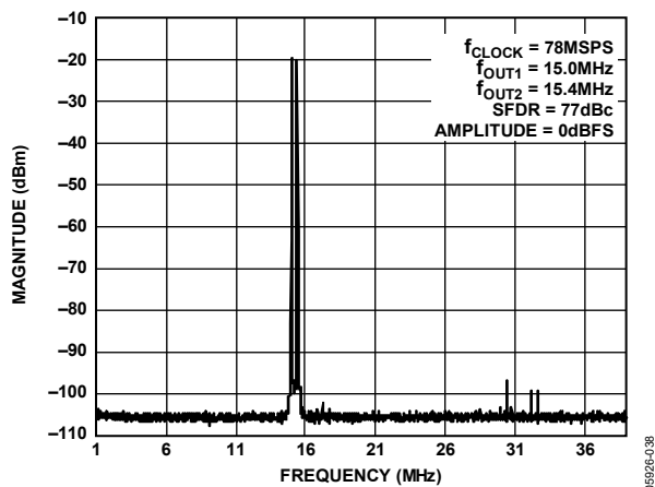
Figure 25. Dual-Tone SFDR
