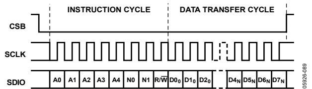
Figure 74. Serial Register Interface Timing, LSB First Write
