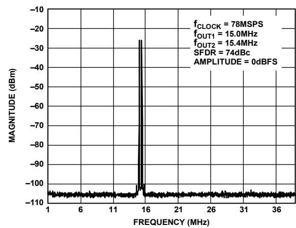
Figure 42. Dual-Tone SFDR
