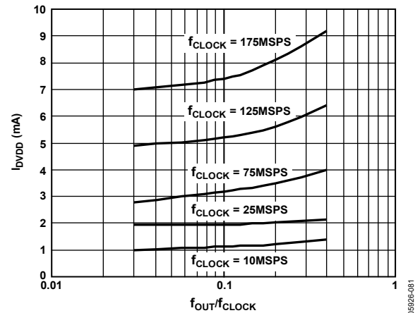
Figure 82. I_{DVDD} vs. f_{OUT}/f_{CLOCK} Ratio at DVDD = 3.3 V
