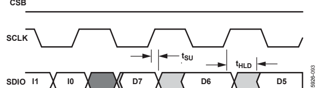
Figure 77. Timing Diagram for SPI Register Read
