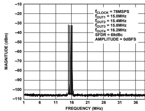
Figure 43. Four-Tone SFDR
