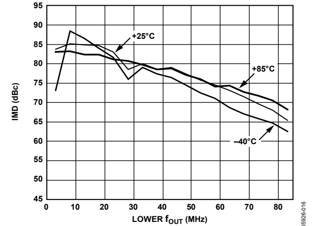
Figure 18. Dual-Tone IMD vs. Lower f_{OUT} and Temperature at 0 dBFS, 175 MSPS
