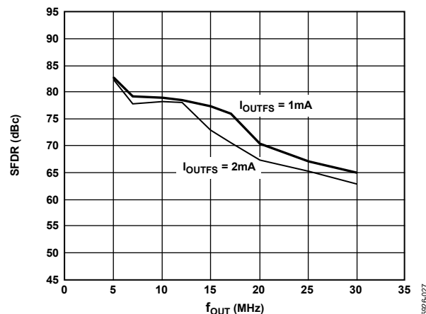
Figure 30. SFDR vs. f_{OUT} and I_{OUTFS} at 65 MSPS
