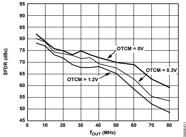
Figure 13. SFDR vs. f_{OUT} and OTCM @ 175 MSPS
