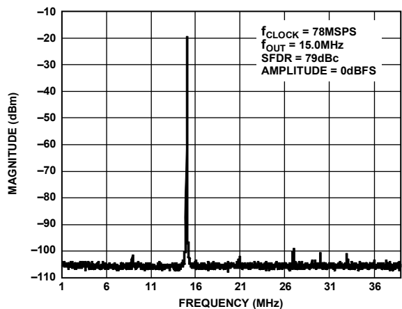
Figure 41. Single-Tone SFDR
