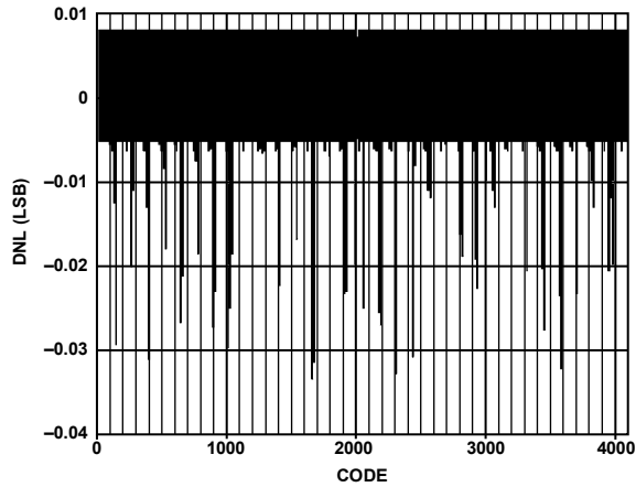
Figure 50. AD9706 Typical Uncalibrated DNL
