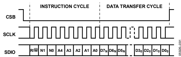
Figure 72. Serial Register Interface Timing, MSB First Write
