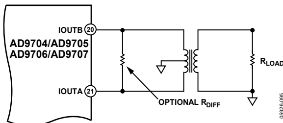
Figure 88. Differential Output Using a Transformer
