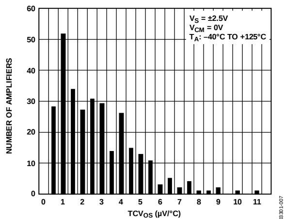
Figure 7. TCV_{OS} Distribution
