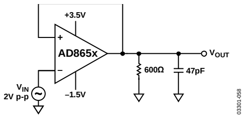
Figure 59. THD + N Test Circuit
