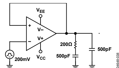
Figure 38. Snubber Network
