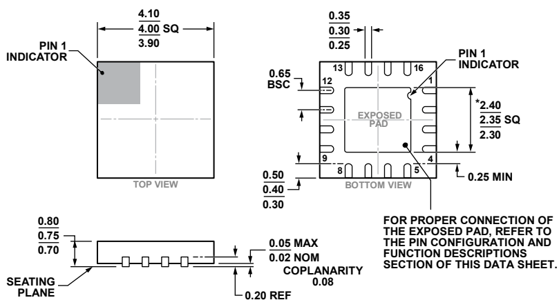
Figure 49. 16-Lead Lead Frame Chip Scale Package [LFCSP] 4 mm x 4 mm Body and 0.75 mm Package Height (CP-16-20)
