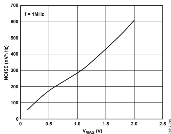
Figure 18. Output Referred Noise vs. V_{MAG} , V_{DDB} = 0.75 V
