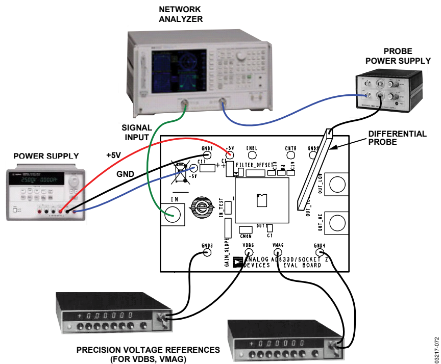
Figure 71. Typical Connections
