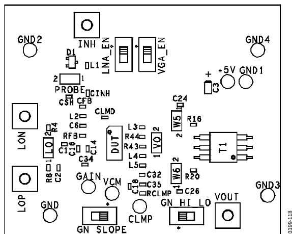
Figure 98. AD8331-EVALZ Assembly
