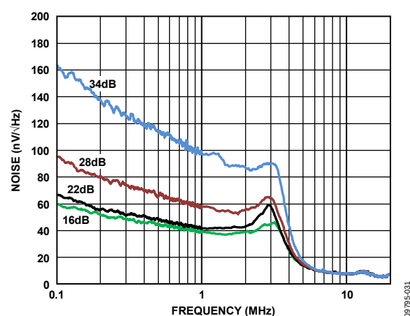
Figure 15. Short-Circuit Output-Referred Noise vs. Frequency
