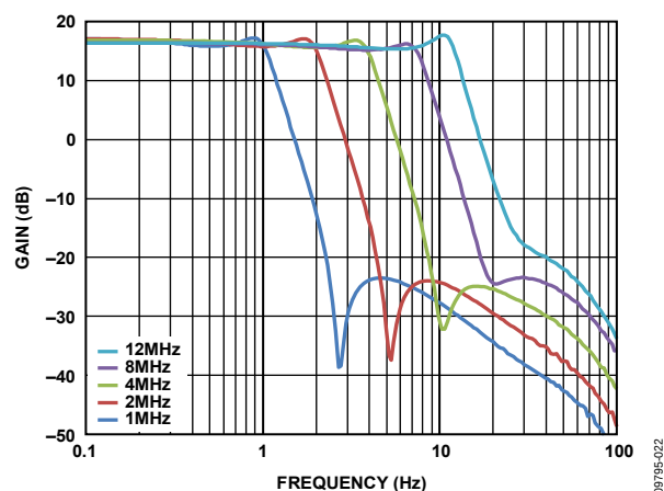
Figure 14. Filter Response
