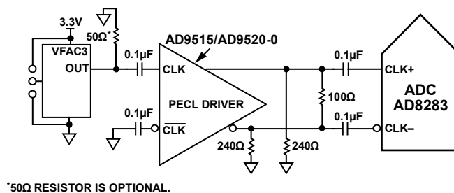
Figure 28. Differential PECL Sample Clock
