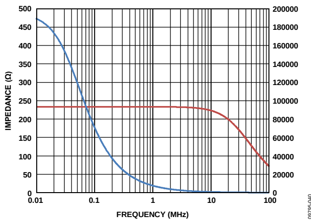
Figure 18. R_{IN} vs. Frequency
