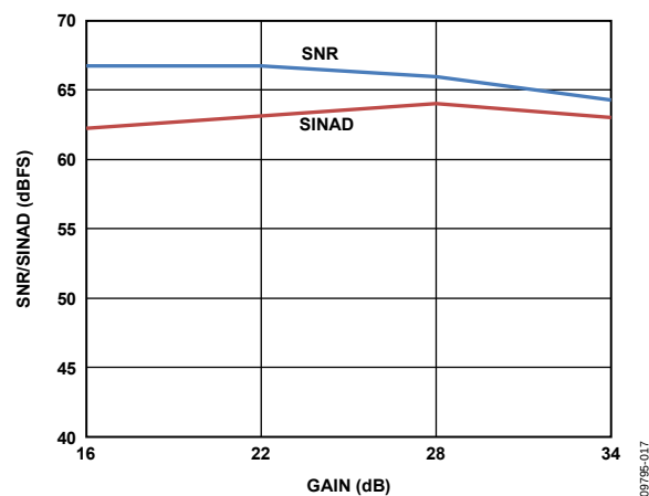
Figure 13. SNR vs. Gain
