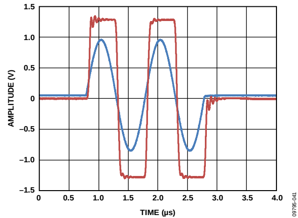
Figure 19. Overdrive Recovery
