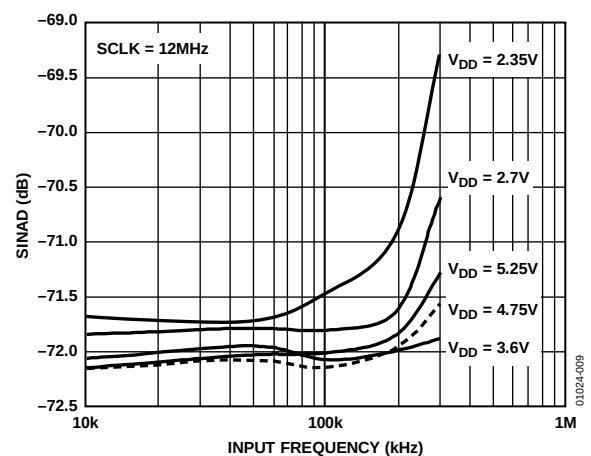
Figure 9. AD7476 SINAD vs. Input Frequency at 605 kSPS
