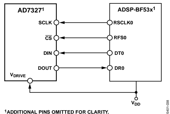
Figure 55. Interfacing the AD7327 to the ADSP-BF53x
