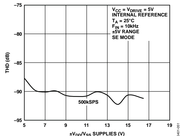
Figure 31. THD vs. \pm V_{DD}/V_{SS} Supply Voltage at 500 kSPS
