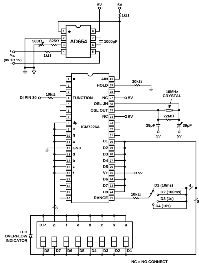
Figure 10. AD654 With Stand-Alone Frequency Counter/ LED Display Driver
