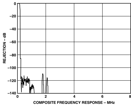
TPC 5. High Decimation AMPS Filter
