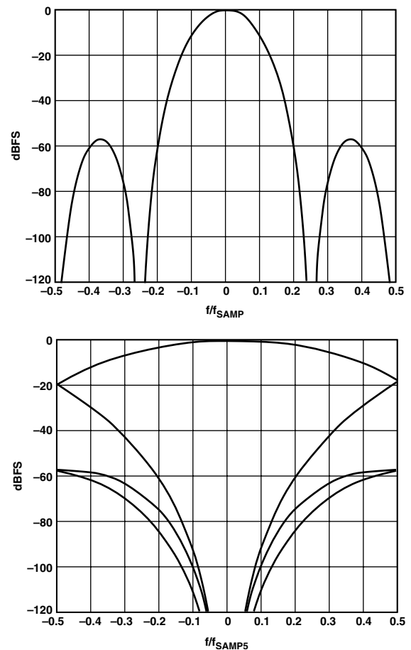
Figure 38. CIC5 Alias Rejection, M_{\text{CIC}5} = 4
