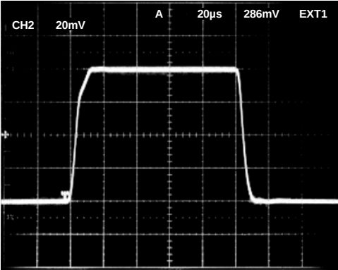
Figure 26. Small Signal Pulse Response, G = +10 , R_L = 20\text{ k}\Omega , C_L = 50\text{ pF}
