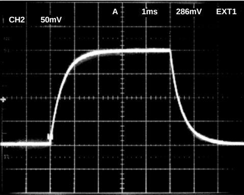
Figure 28. Small Signal Pulse Response, G = +1000 , R_L = 20\text{ k}\Omega , C_L = 50\text{ pF}
