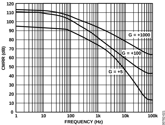
Figure 23. CMRR vs. Frequency, \pm 5\text{ V}_S ( CMV = 200\text{ mV p-p} )
