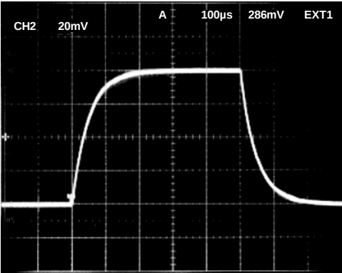
Figure 27. Small Signal Pulse Response, G = +100 , R_L = 20\text{ k}\Omega , C_L = 50\text{ pF}
