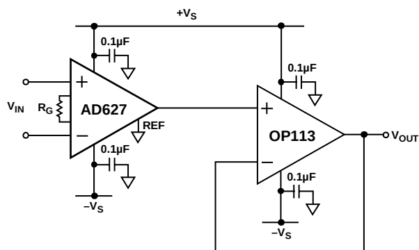
Figure 40. Output Buffering
