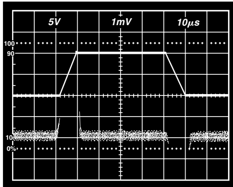
TPC 19. Large Signal Pulse Response and Settling Time Gain, G = 10 ( 0.5 mV = 0.01\% ), R_L = 1 k\Omega , C_L = 100 pF
