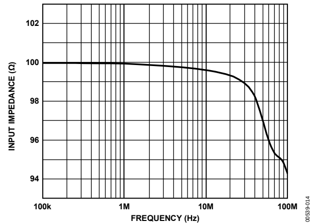
Figure 15. Input Impedance vs. Frequency (Gain = -10 dB)
