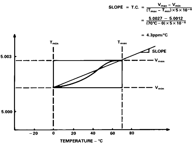
Figure 9. Typical AD586L Temperature Drift
