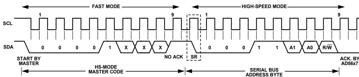
Figure 56. Placing the AD5627R/AD5667R in High Speed Mode
