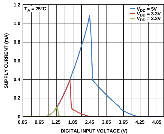
Figure 13. Supply Current ( I_{DD} ) vs. Digital Input Voltage
