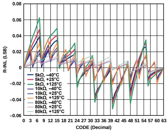
Figure 8. R-INL vs. Code
