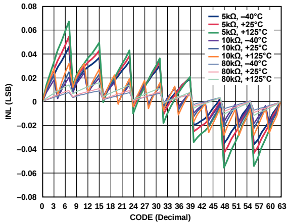
Figure 9. INL vs. Code
