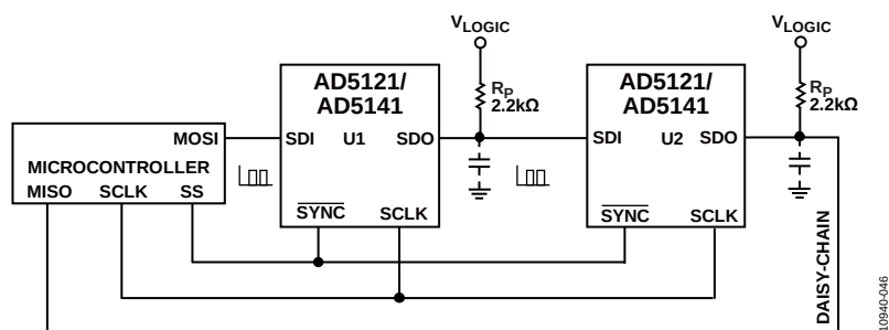
Figure 40. Daisy-Chain Configuration
