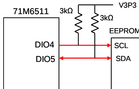
Figure 33: EEPROM Connection
