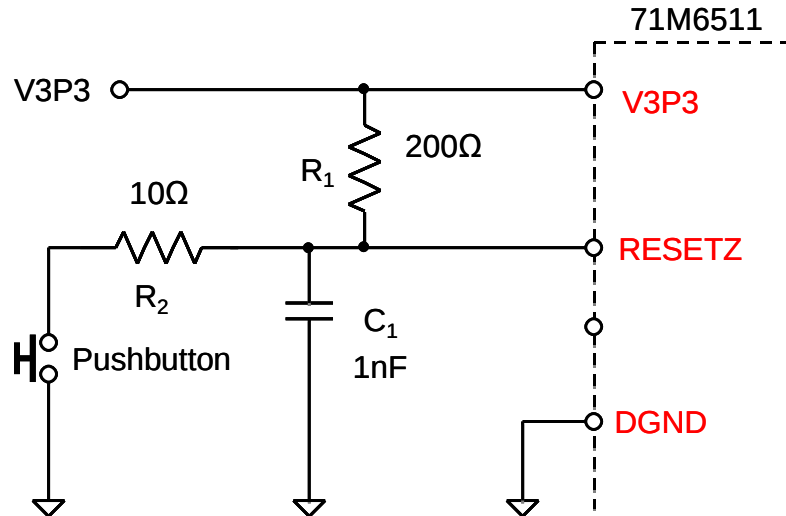
Figure 37: External Components for RESETZ
