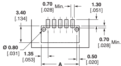
PCB Mounting Layout
