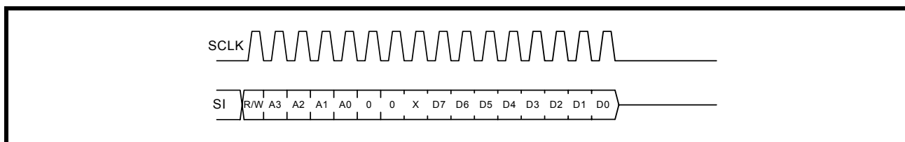
FIGURE 7. SPI WRITE
