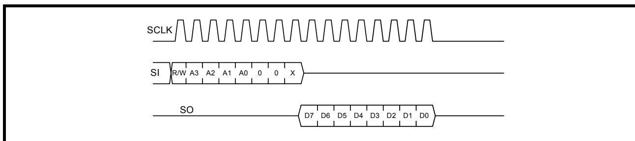
FIGURE 8. SPI READ
