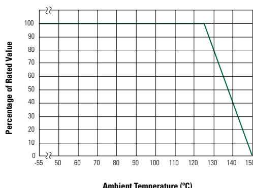
Figure 1B - Power Derating for Phenolic Coated
