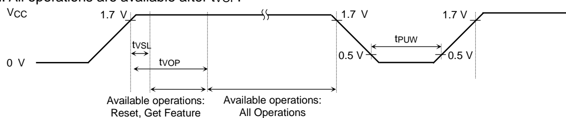
Figure 10. Power ON/OFF Timing
