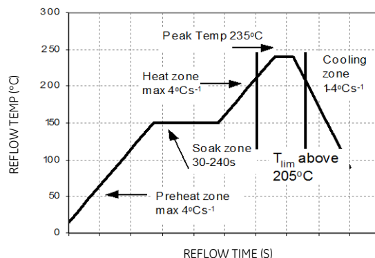
Figure 55. Time Limit, T_{lim} , Curve Above 205^{\circ}\text{C} Reflow .
