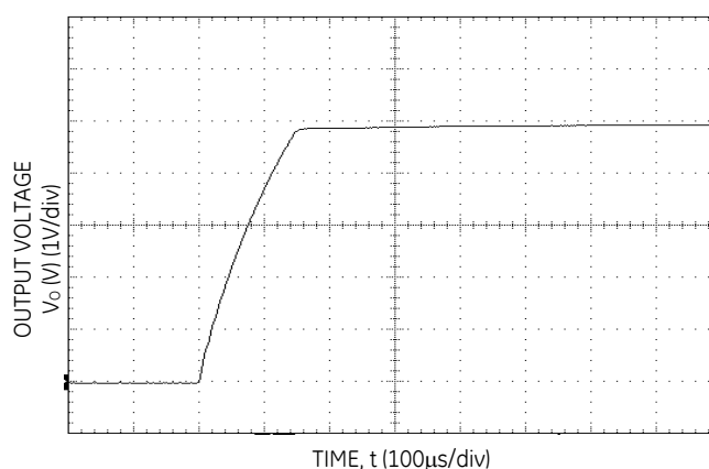
Figure 36. Typical Start-Up Output Voltage Rise Characteristic.
