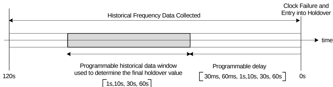
Figure 12. Programmable Holdover Window
