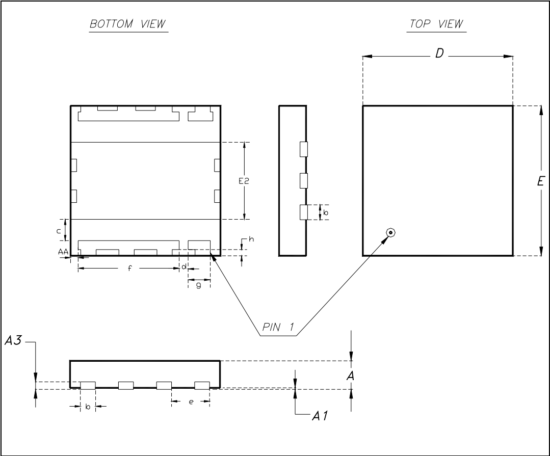
Figure 6. Package dimensions
