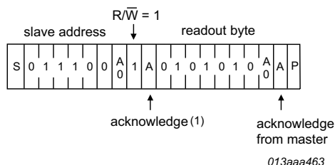
Fig 25. I 2 C-bus protocol read mode
