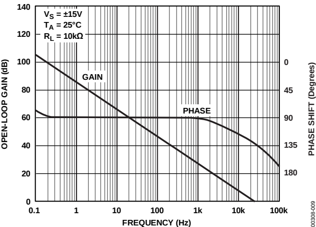
Figure 9. Open-Loop Gain and Phase Shift vs. Frequency
