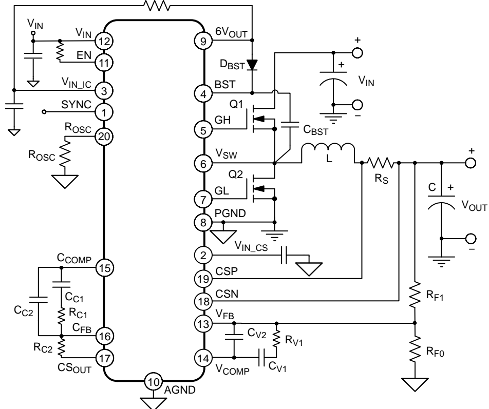
Figure 2. Application Schematic
