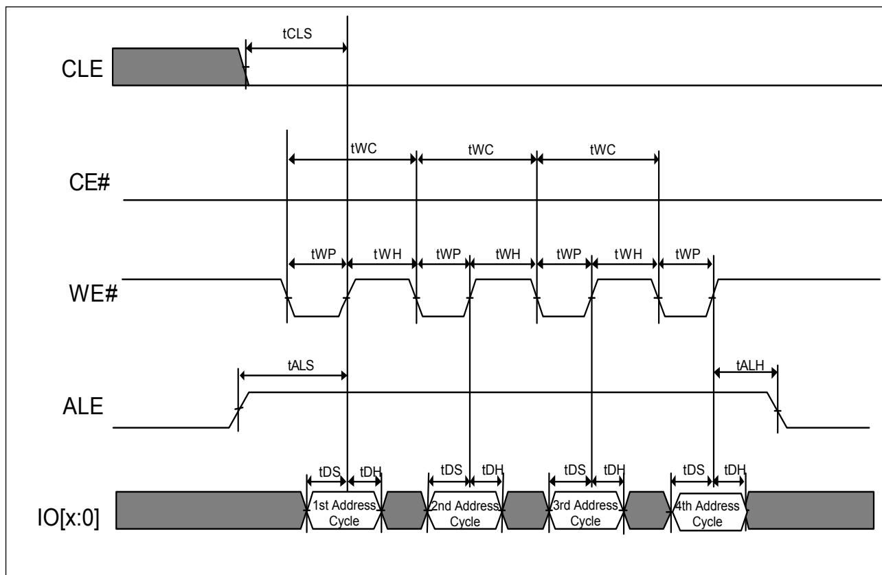
Figure 3. AC Waveforms for Address Input Cycle
