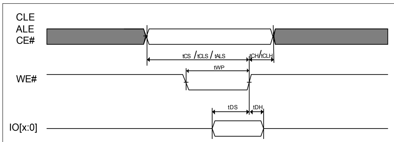
Figure 3. AC Waveforms for Address Input Cycle
