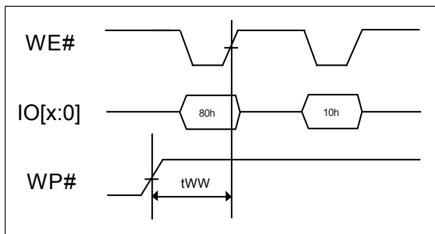
Figure 38-1. Enable Programming of WP# Signal
