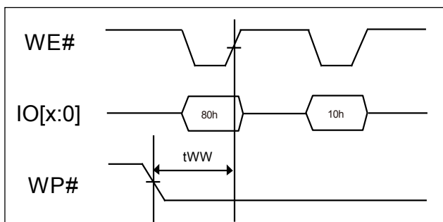
Figure 38-2. Disable Programming of WP# Signal
