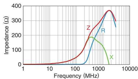
MMZ1608D500CTAH0
