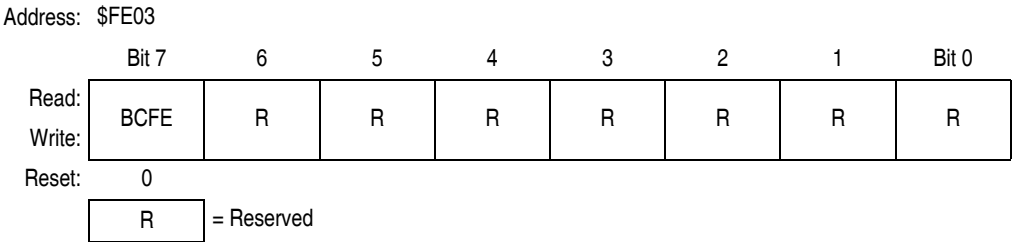
Figure 15-8. Break Flag Control Register (BFCR)
