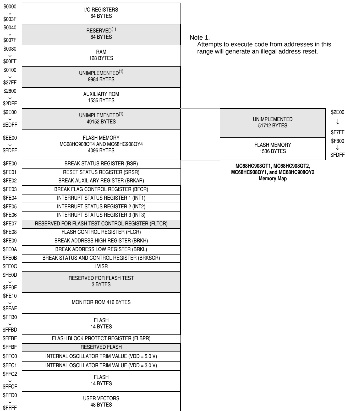
Figure 2-1. Memory Map
