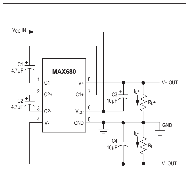
Figure 1. Test Circuit
