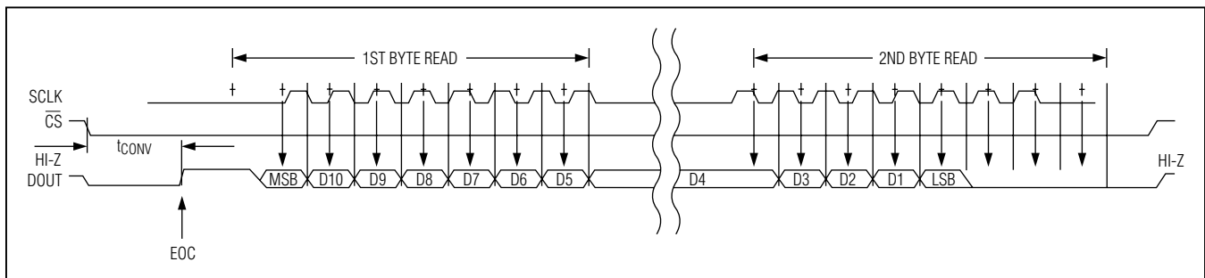
Figure 14. SPI/MICROWIRE Serial Interface Timing (CPOL = CPHA = 0)
