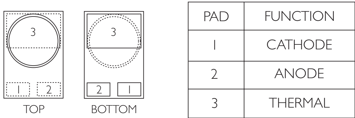
Figure 9a. LUXEON Rebel Color Line pad configuration.
